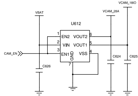
<CAM LDO>
