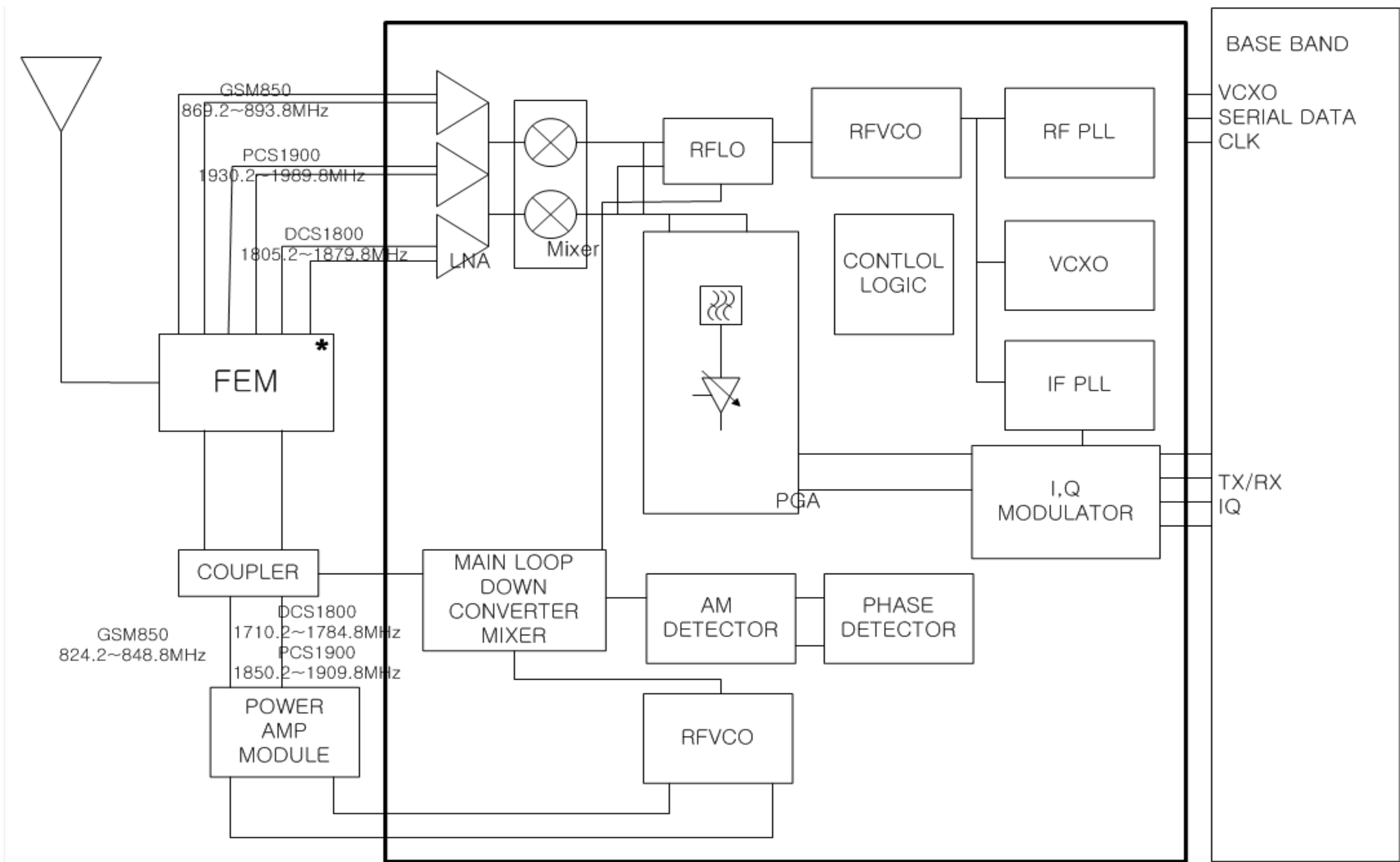
9-1. RF Solution Block Diagram
