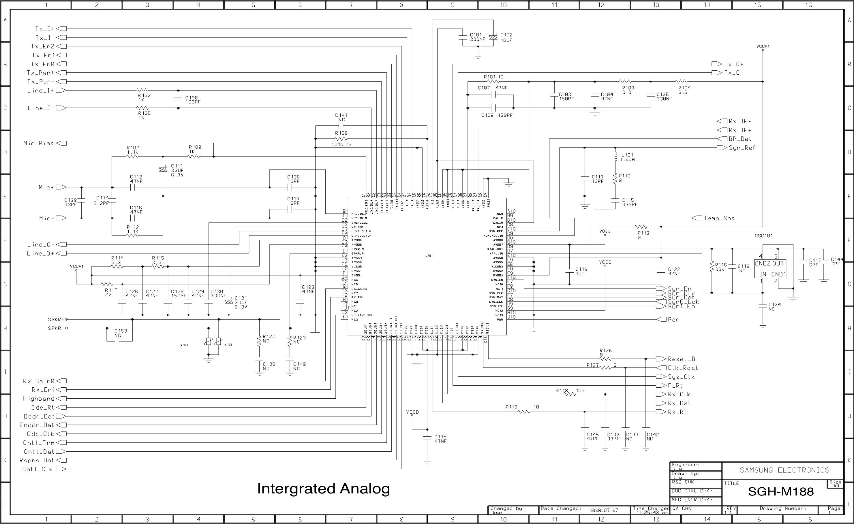
5-1 SGH-M188 Intergrated Analog Circuit Diagram
