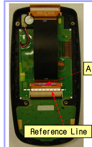
MAIN FPCB
