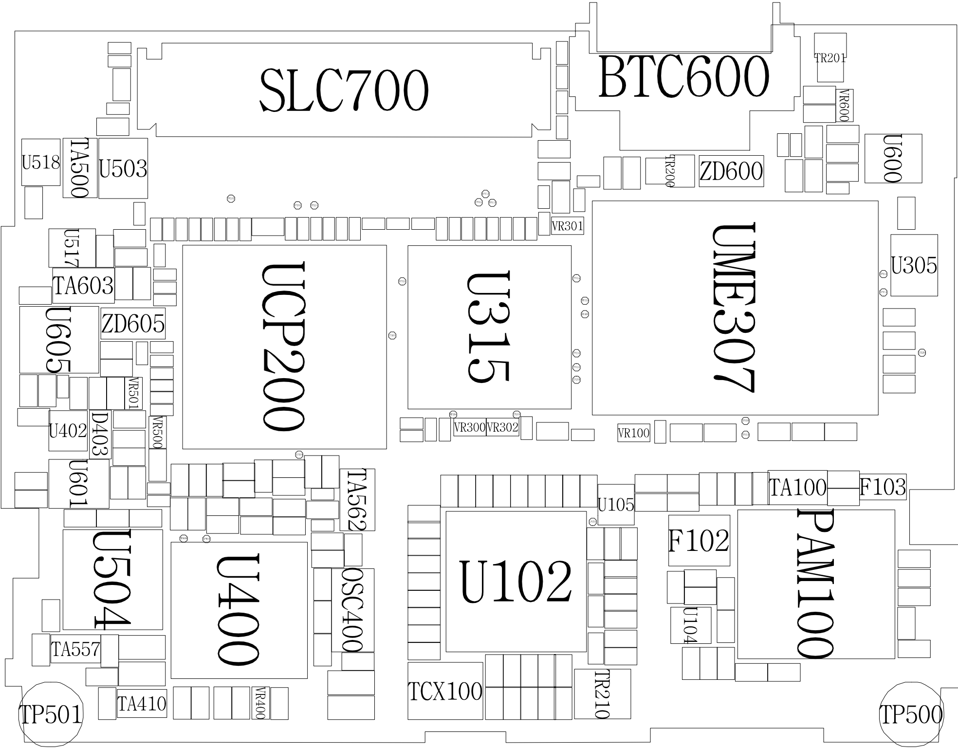
6-1. Main PCB Top Diagram
