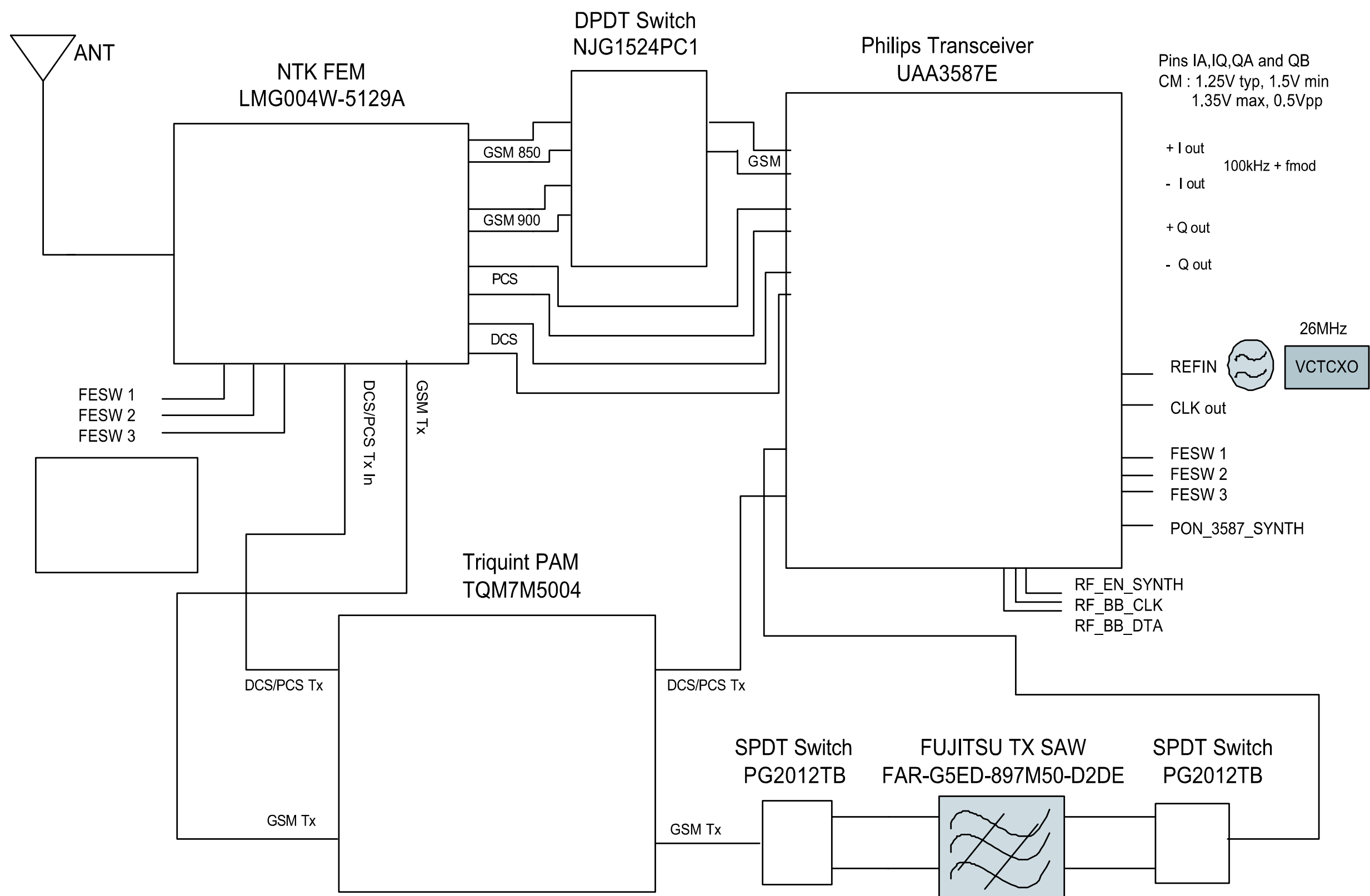
5-1. RF Solution Block Diagram
