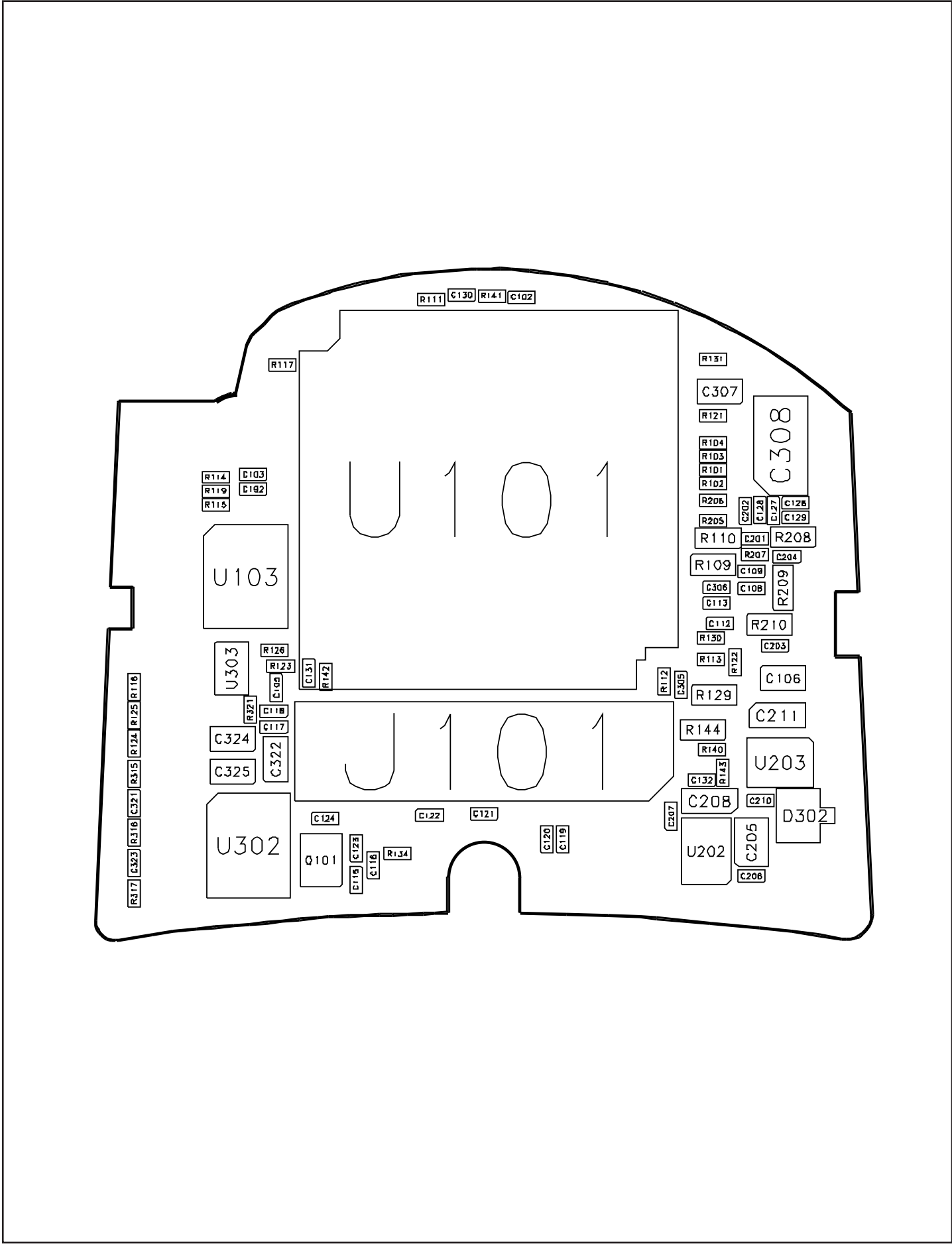
4-5 Memory PCB Bottom Diagram
