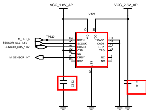
Magnetic Sensor
