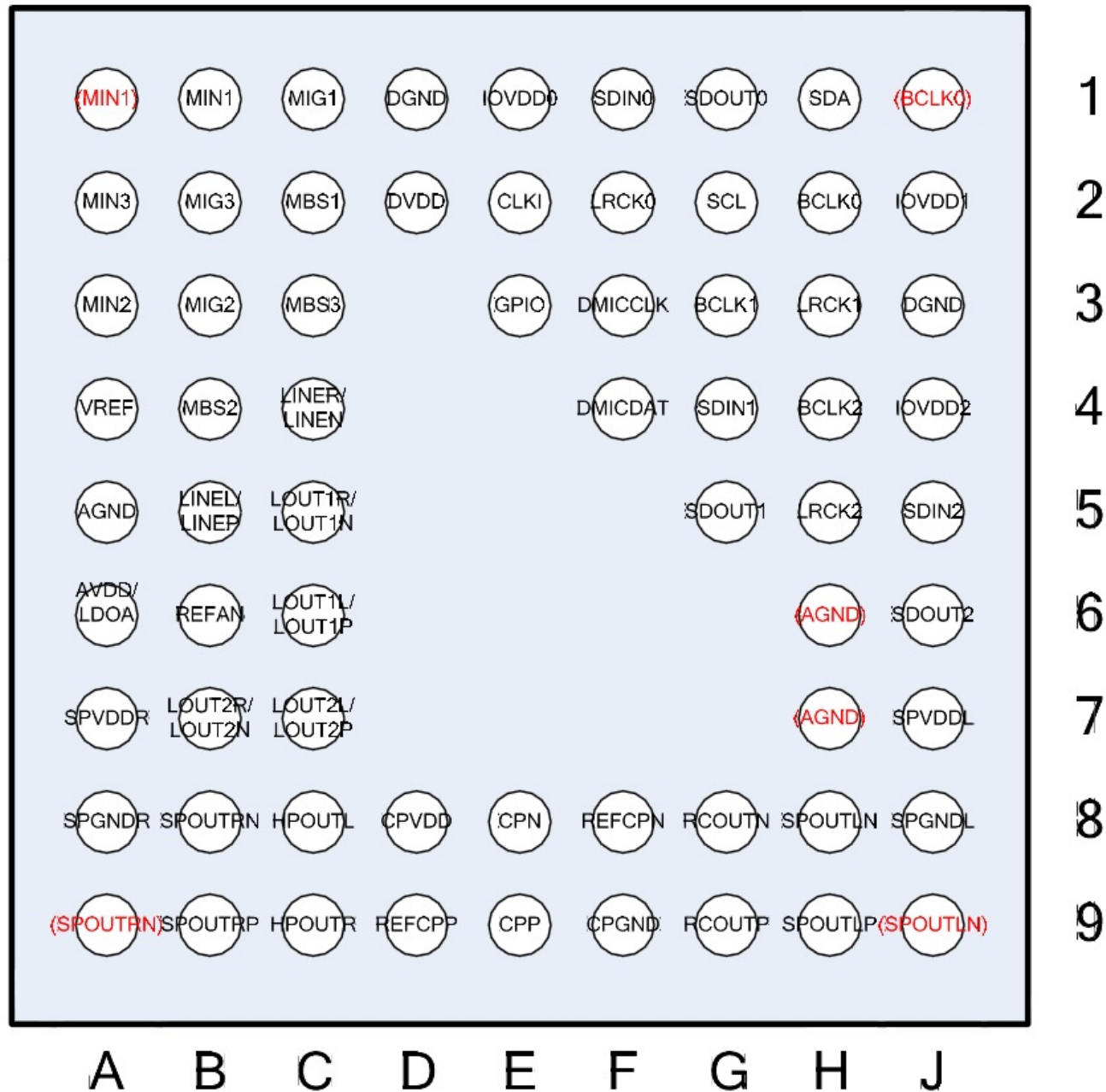
67-ball WLCSP Bottom VIEW
