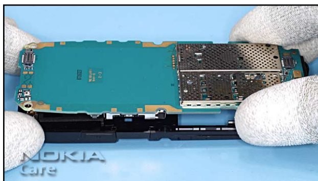
14. Remove the PWB from the B-COVER.
