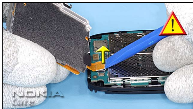
10. Gently open the UI MODULE connector, paying attention to the surrounding components.
