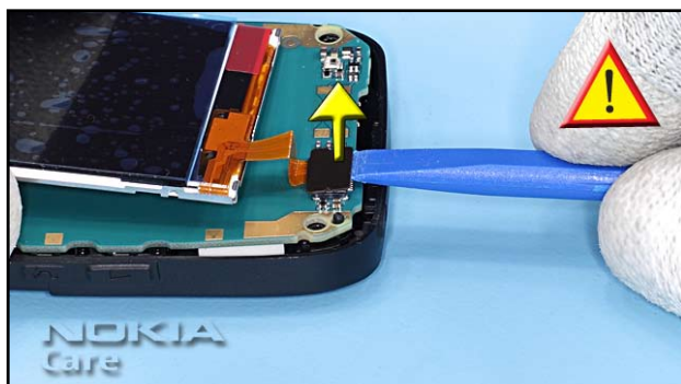
12. Gently open the DISPLAY connector, paying attention to the surrounding components.
