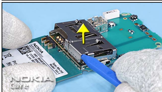
16. Remove the CARD SHIELD.
