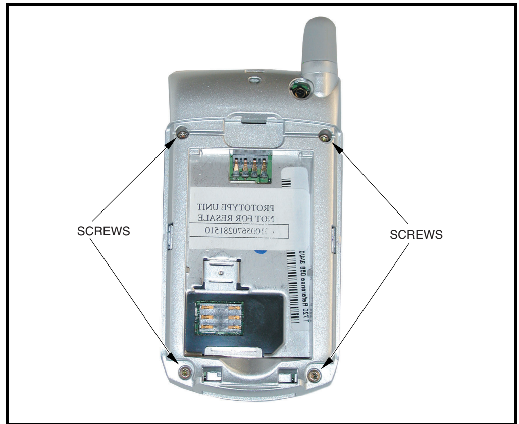
Figure 8. Removing the Rear Housing Assembly Screws
