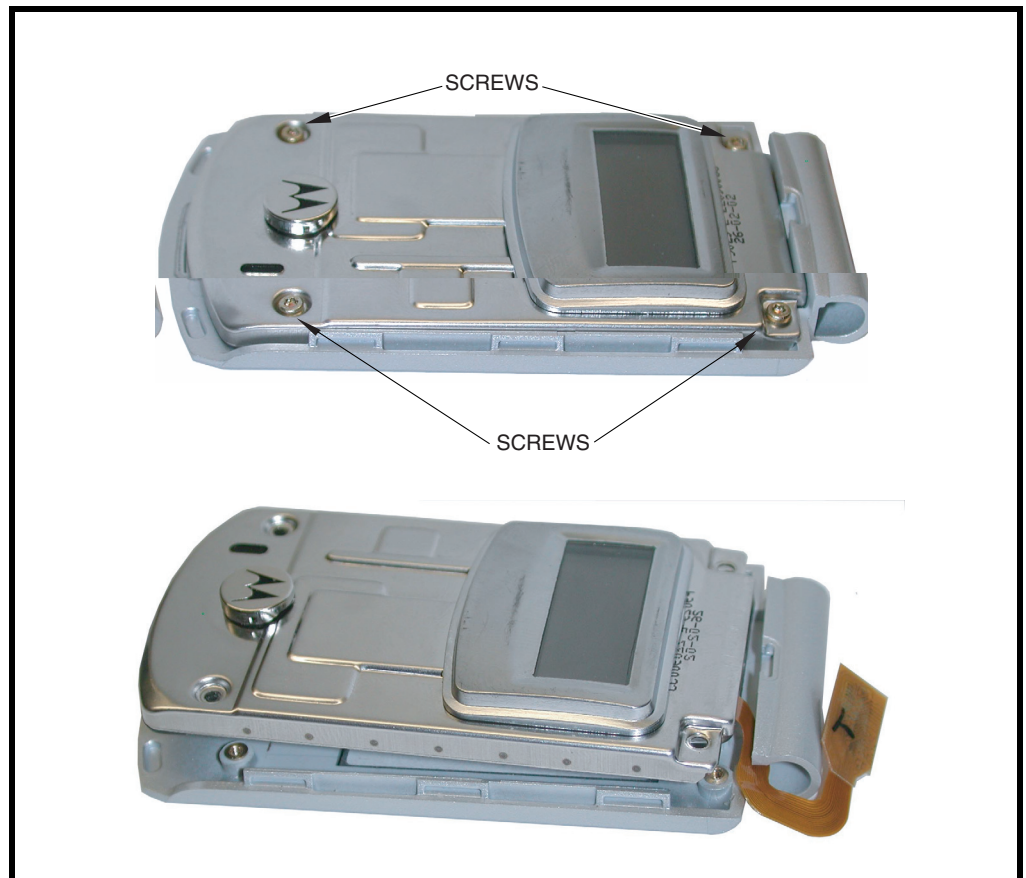
Figure 18. Removing the Display Module
