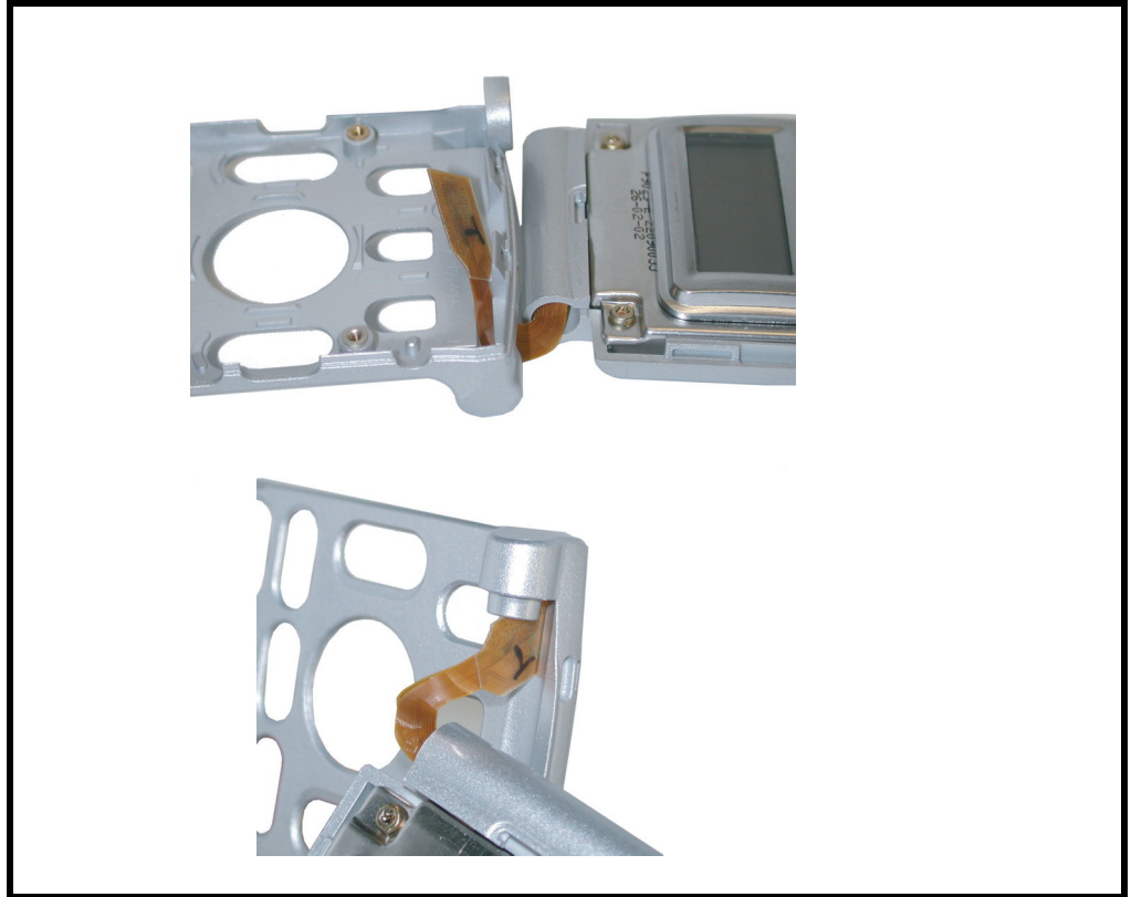
Figure 16. Removing the Flex Connector
