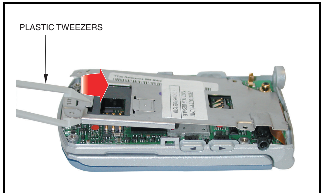
Figure 10. Removing the Chassis Shield
