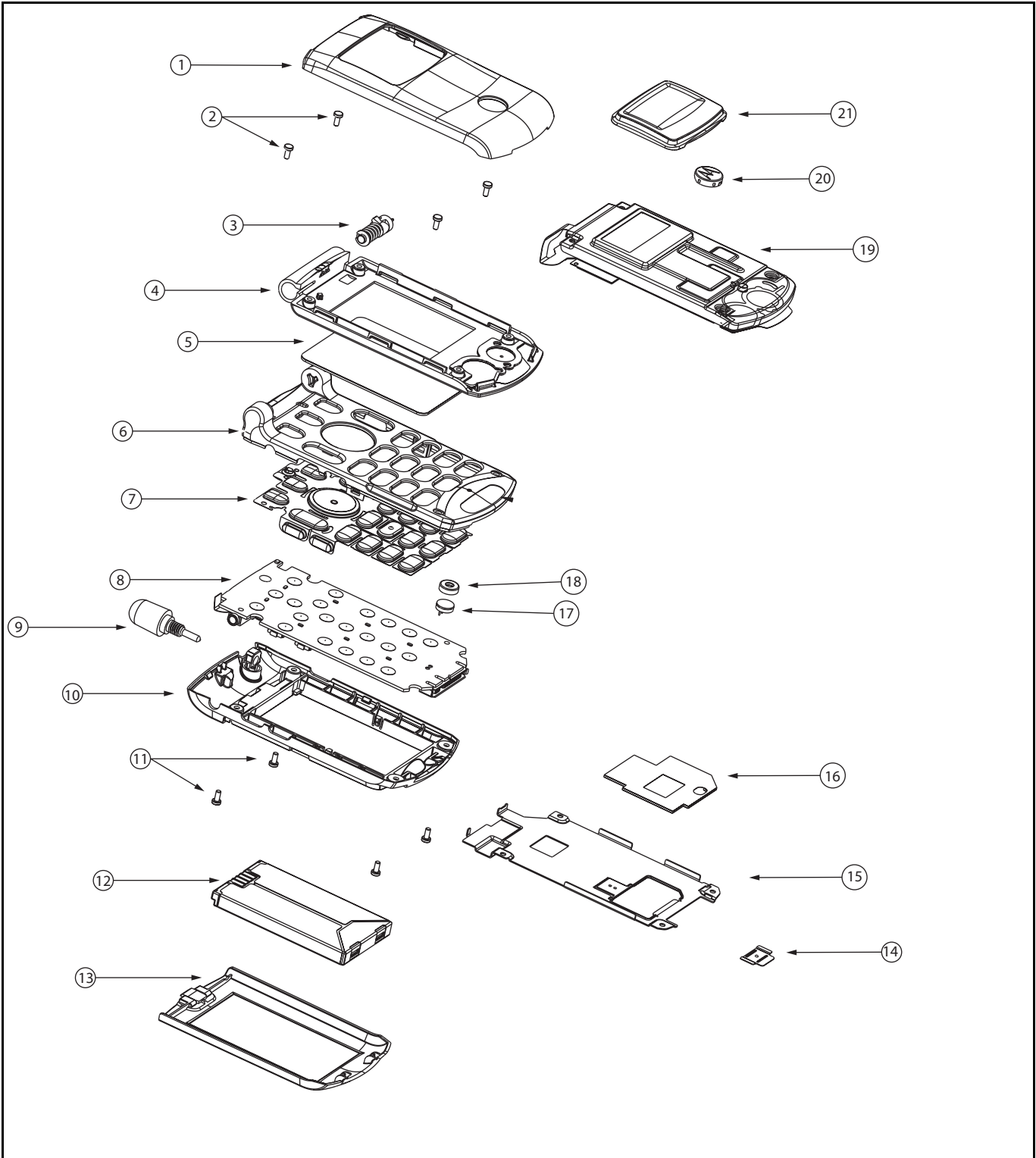
Figure 21. Exploded View
