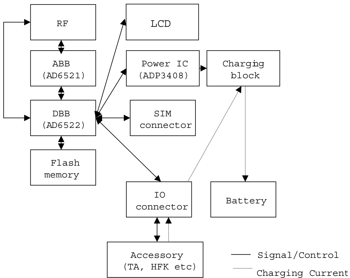
Figure 7-1. block diagram
