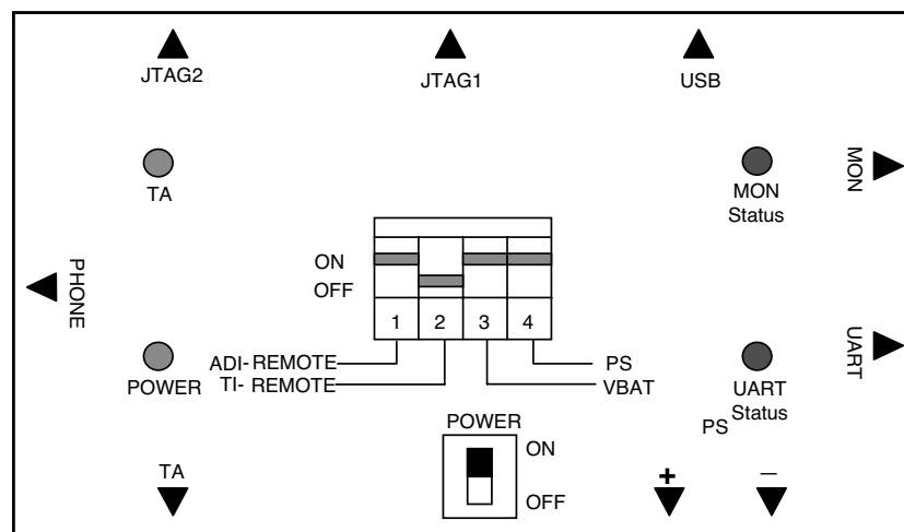
Figure 11-1 The top view of Test JIG
