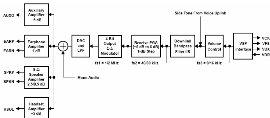
Figure 21. Voice Downlink path Block Diagram
