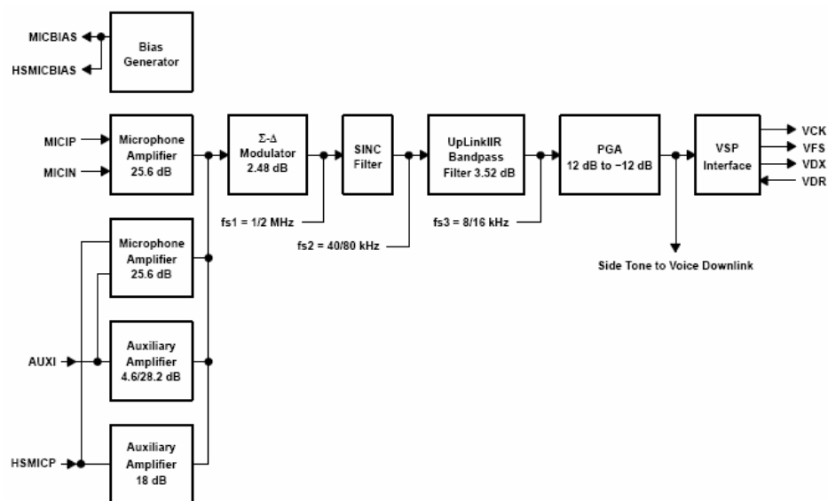
Figure 20. Voice Uplink path Block Diagram
