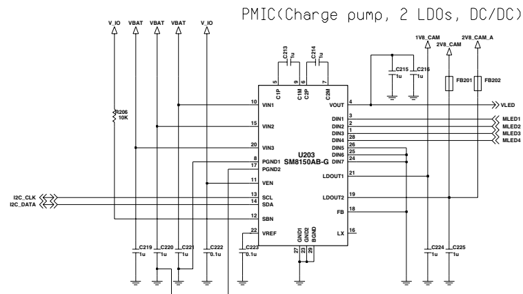
Figure 18. LCD Back-light driving ckts
