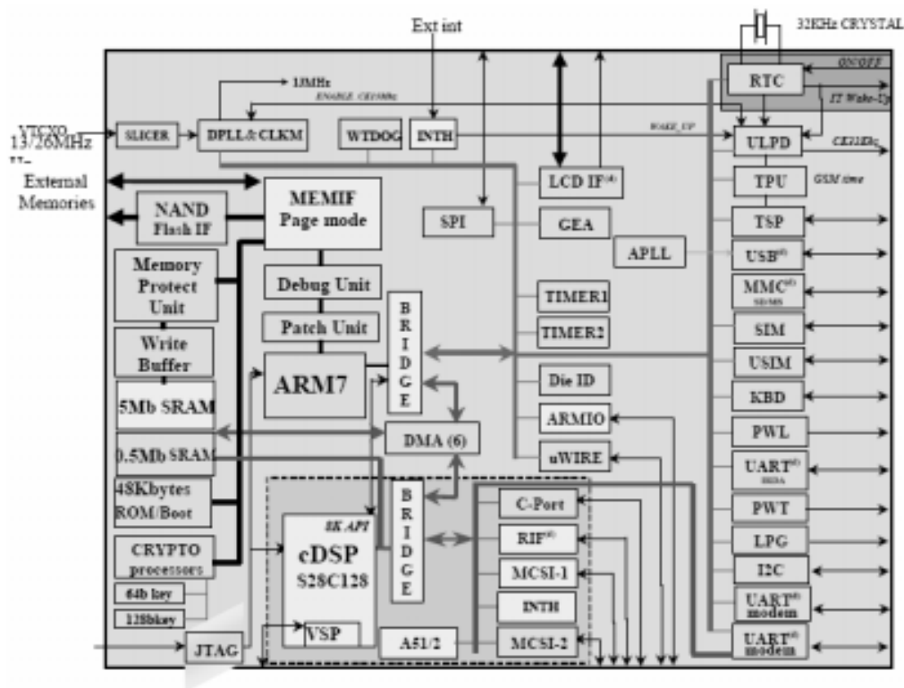
Figure 7. Top level block diagram of the Calypso-Plus
