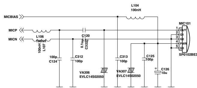
Figure 14. Main Mic. Circuits.
