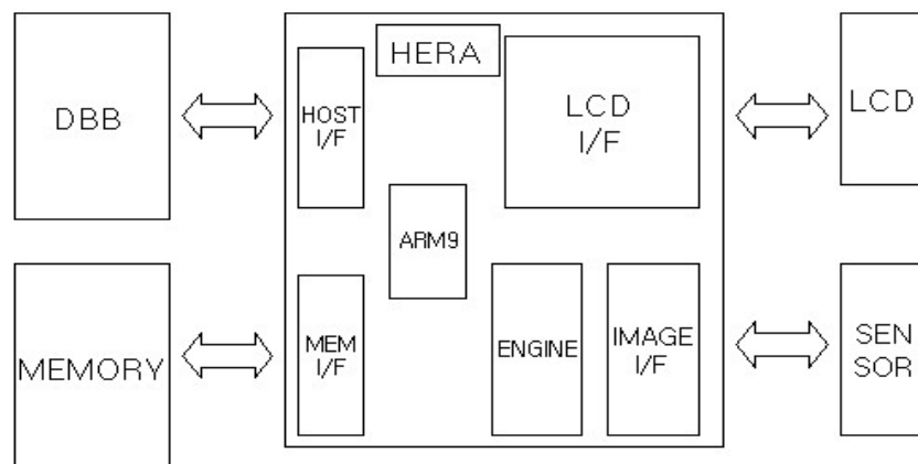
Figure 24. LCD scheme
