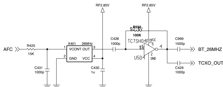
Figure 4. VC-TCXO Circuit
