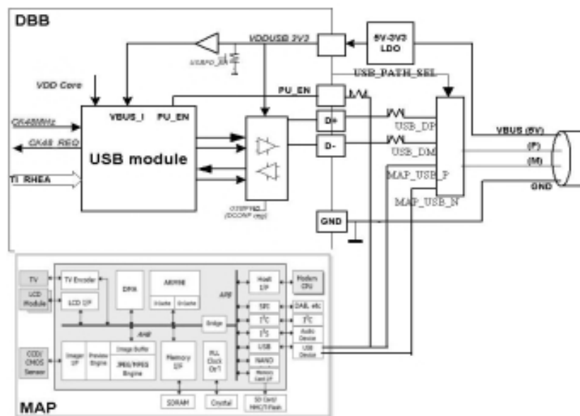
Figure 9. USB interface diagram
