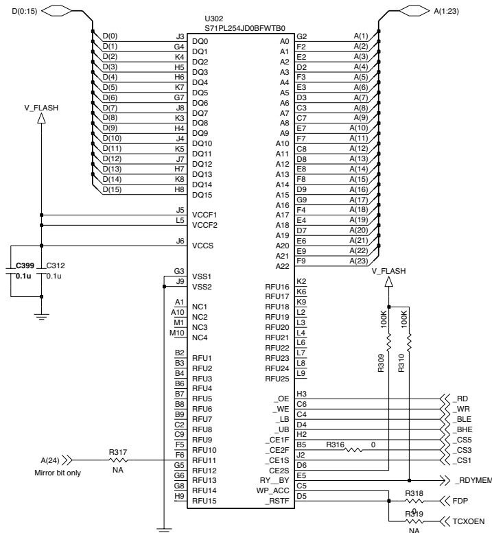
Figure 7. Memory interface scheme
