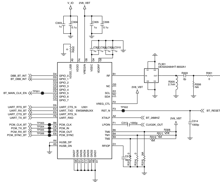
Figure 26. Bluetooth I/F
