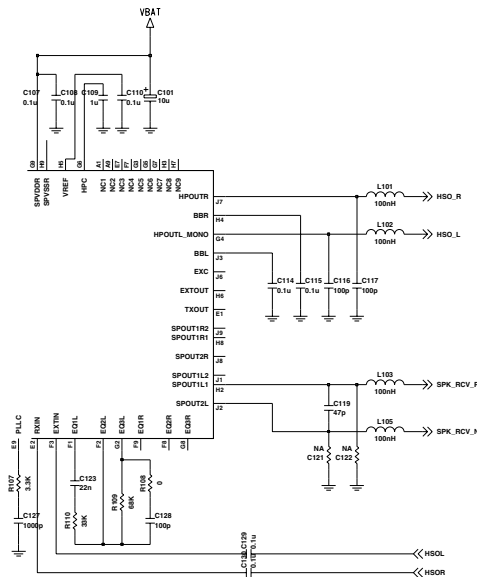
Figure 15. Down-link circuits related with YMU783
