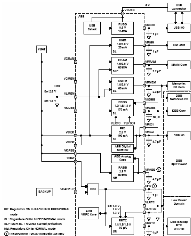
Figure 23. Power Supply Scheme
