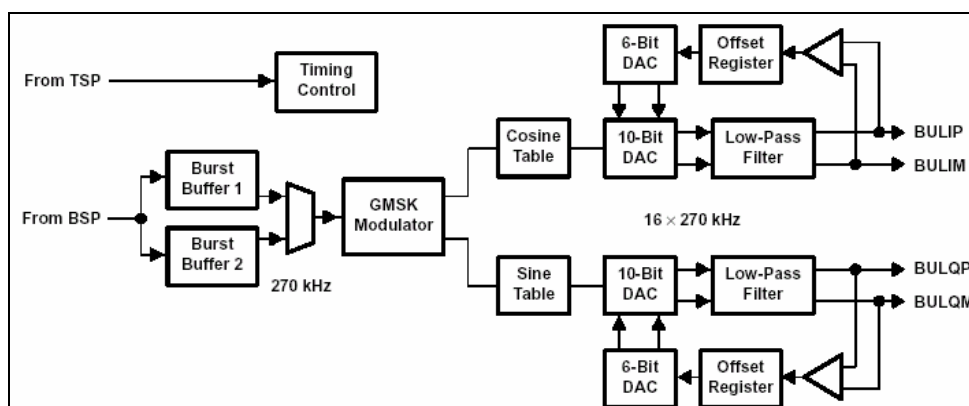
Figure 22. Baseband Codec Block Diagram
