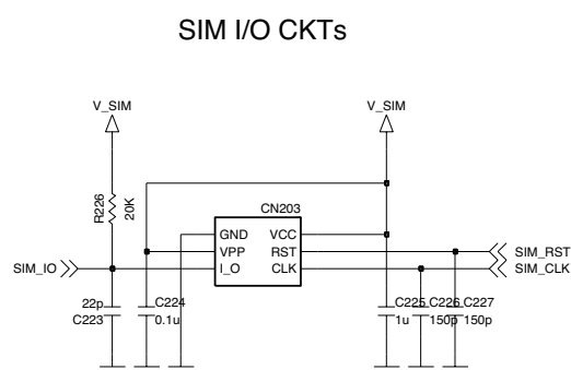
Figure 8. SIM Interface
