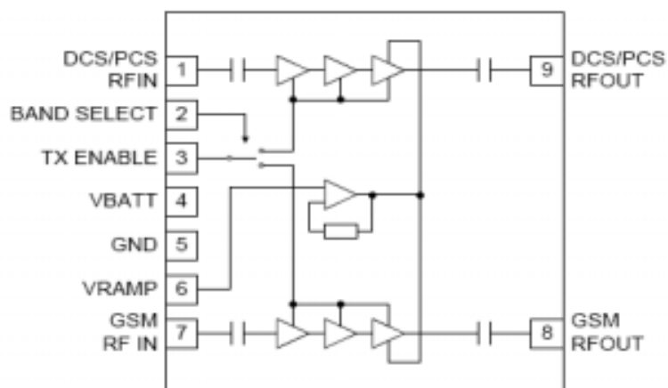
Figure 4. POWER AMP
