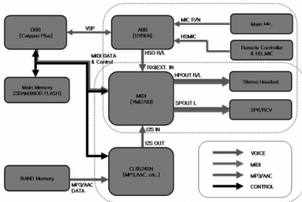
Figure 10. Audio Block Diagram
