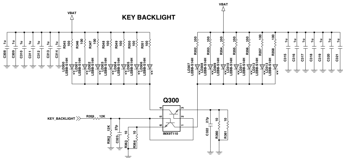
Figure 3-15. KEY BACK-LIGHT ILLUMINTION
