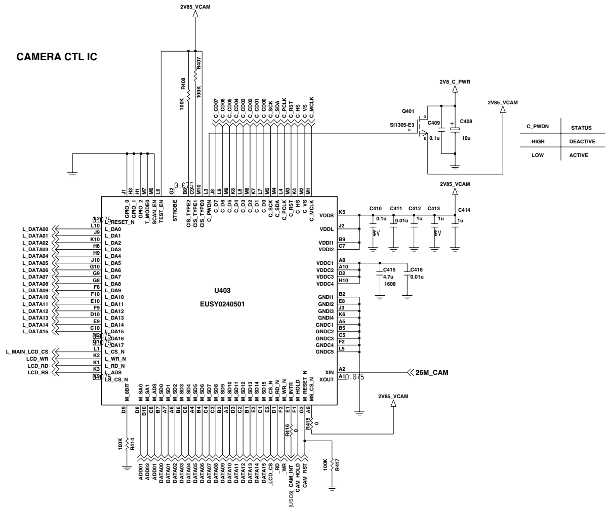
Figure 3-10. CL761A CIRCUIT
