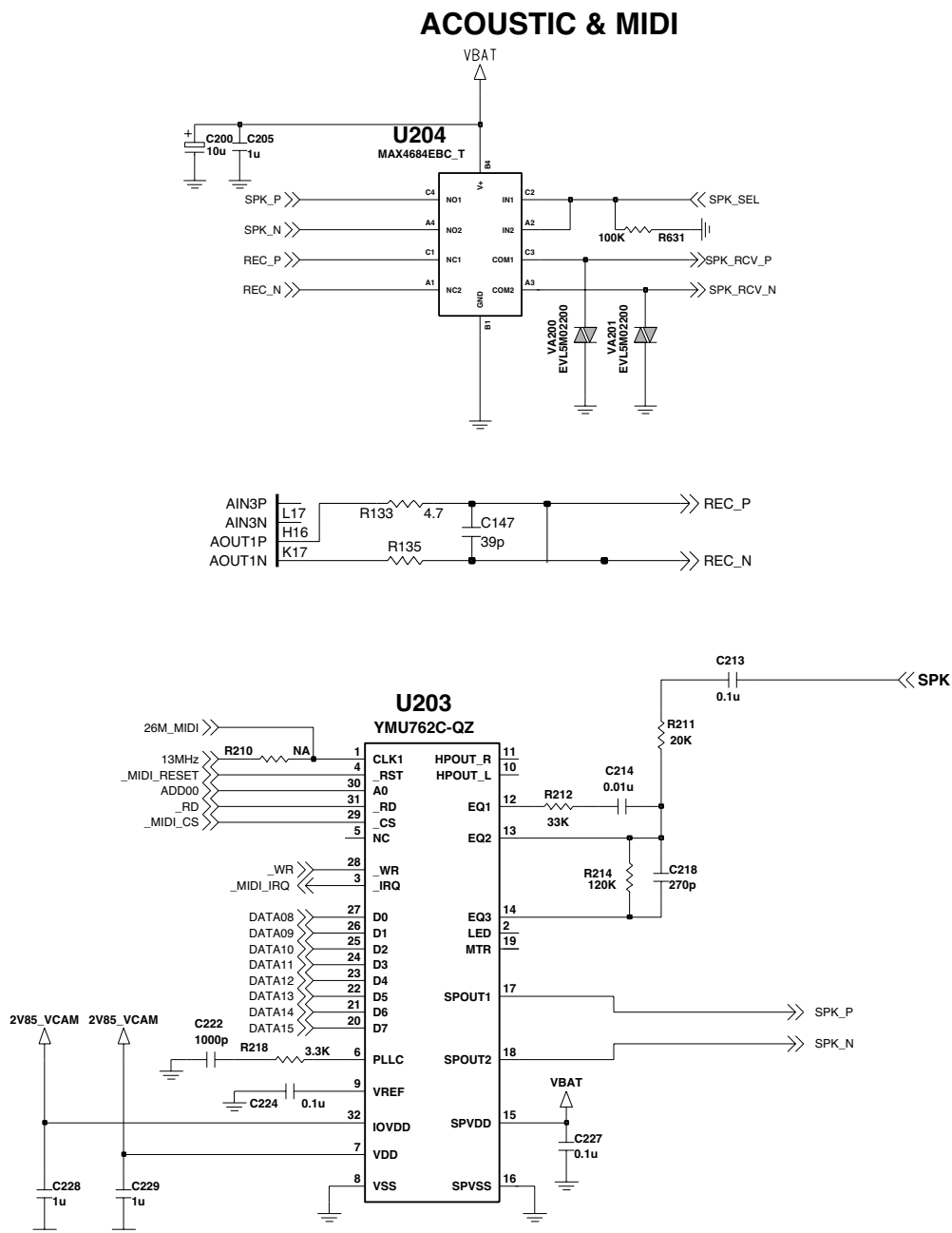
Figure 3-13. MAIN SPEAKER
