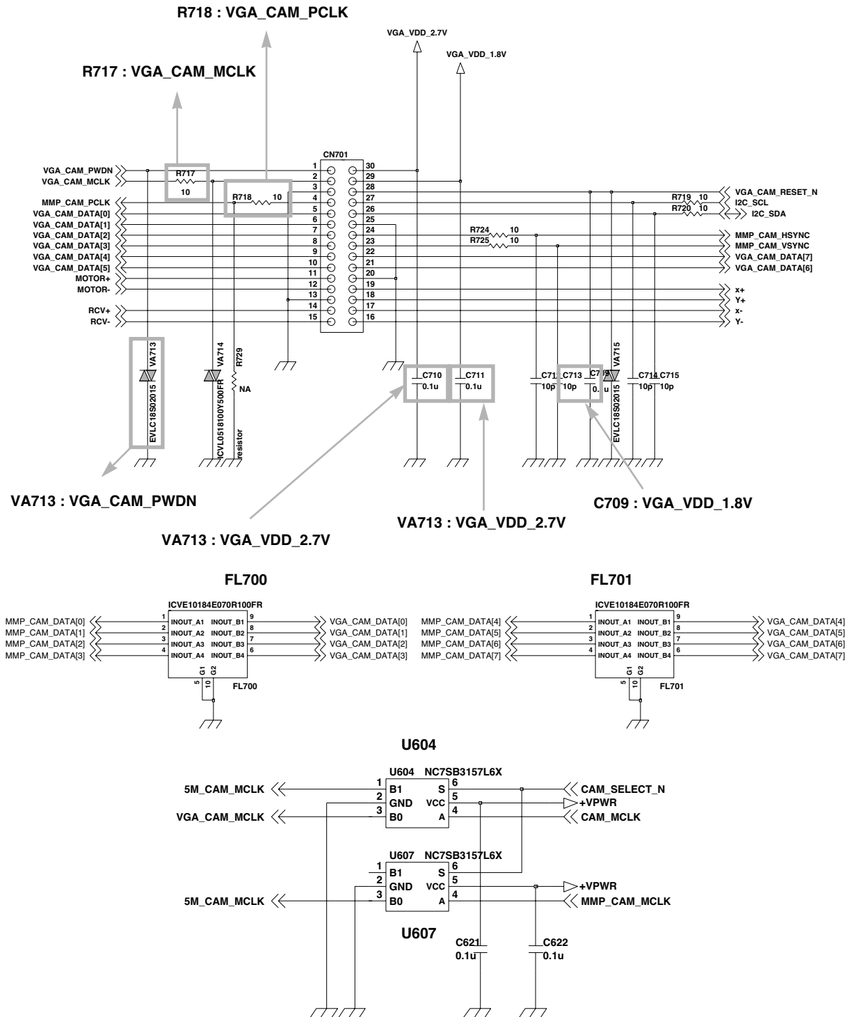
Schematic of VGA camera part
