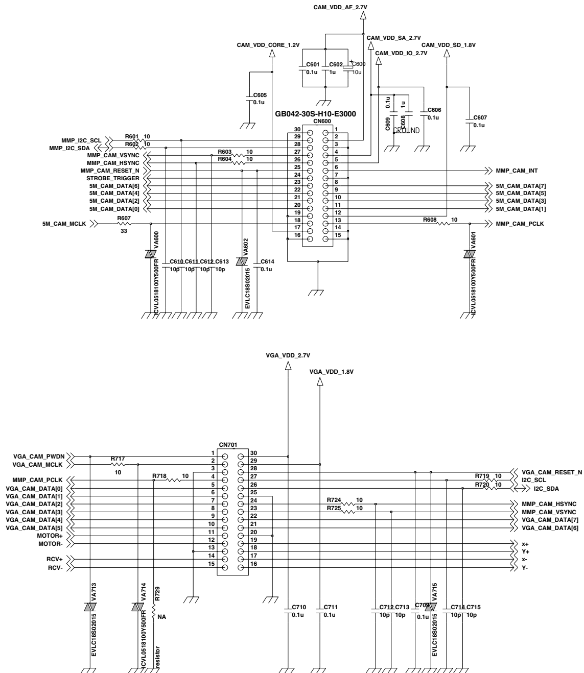
Figure. Camera PCB Board to Board Connector
