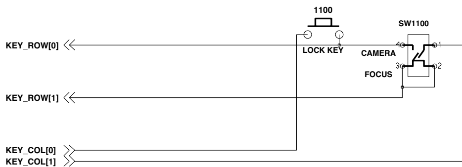
Figure. Side Keypad Circuit
