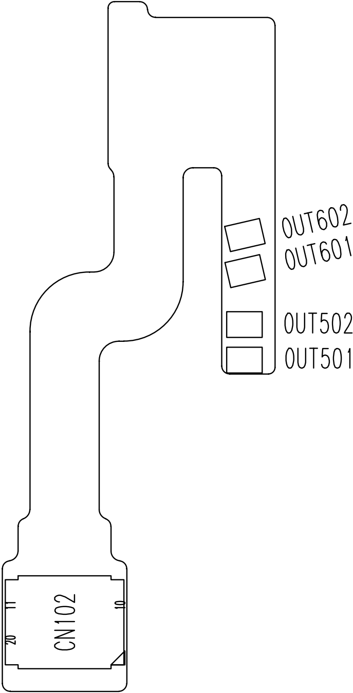
KU990-F-CAM-1.0-B0T
