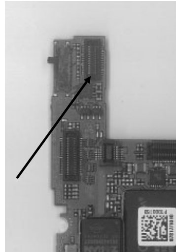
VGA CAM FPCB connector
