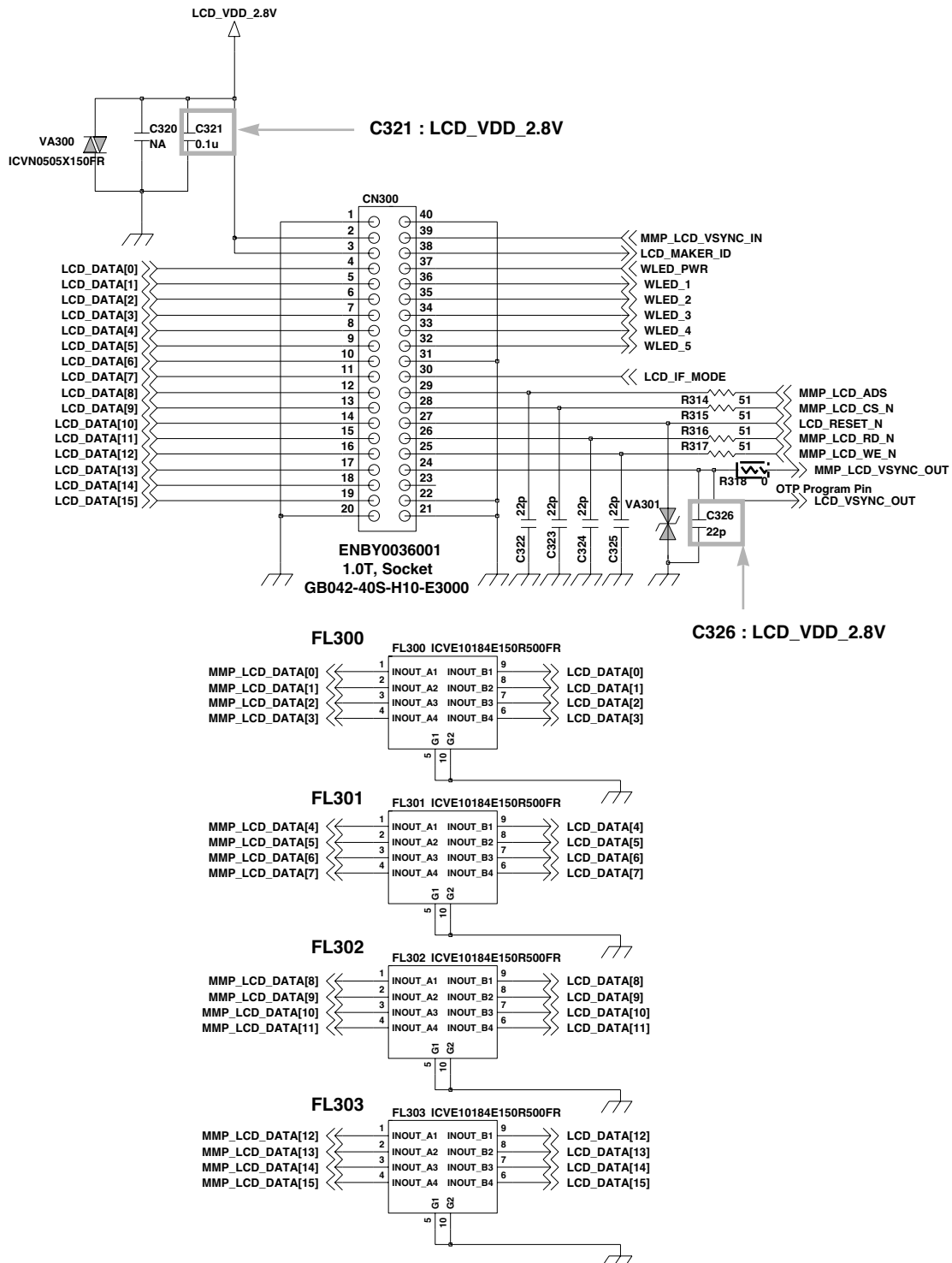
Schematic of LCD part
