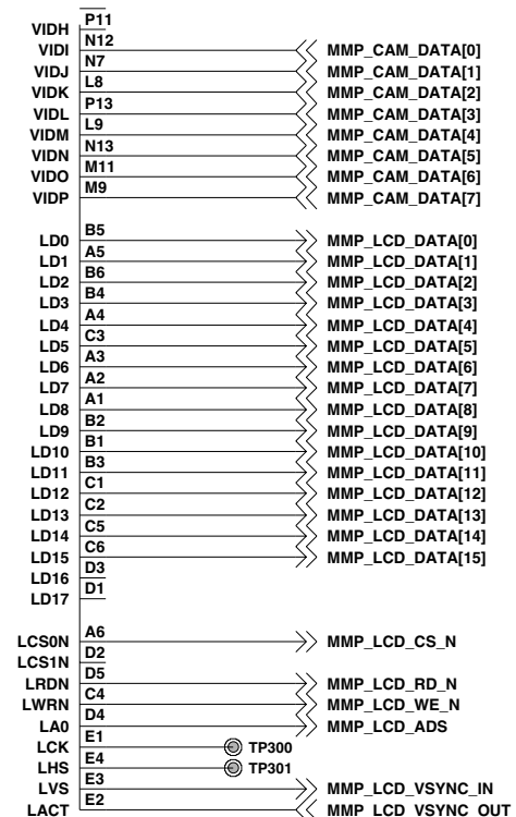
[ Schematics ]
