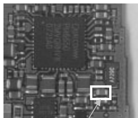
C552(VREG_USIM_3.0V)
