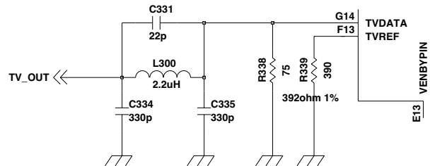
[ Schematics ]
