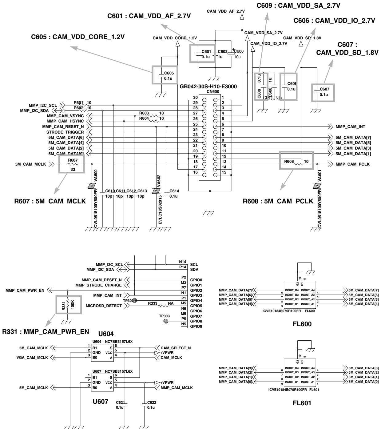
Schematic of 5M camera part
