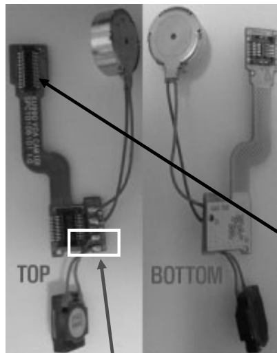
Receiver
