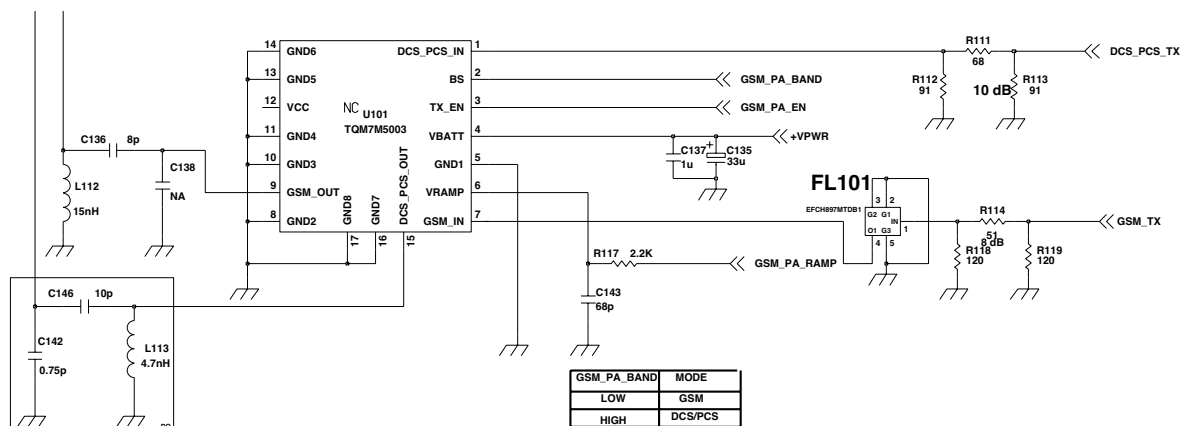
[Figure 1. 8] GSM PAM Schematic
