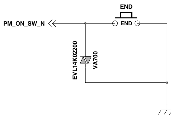
Figure. END Keypad Circuit
