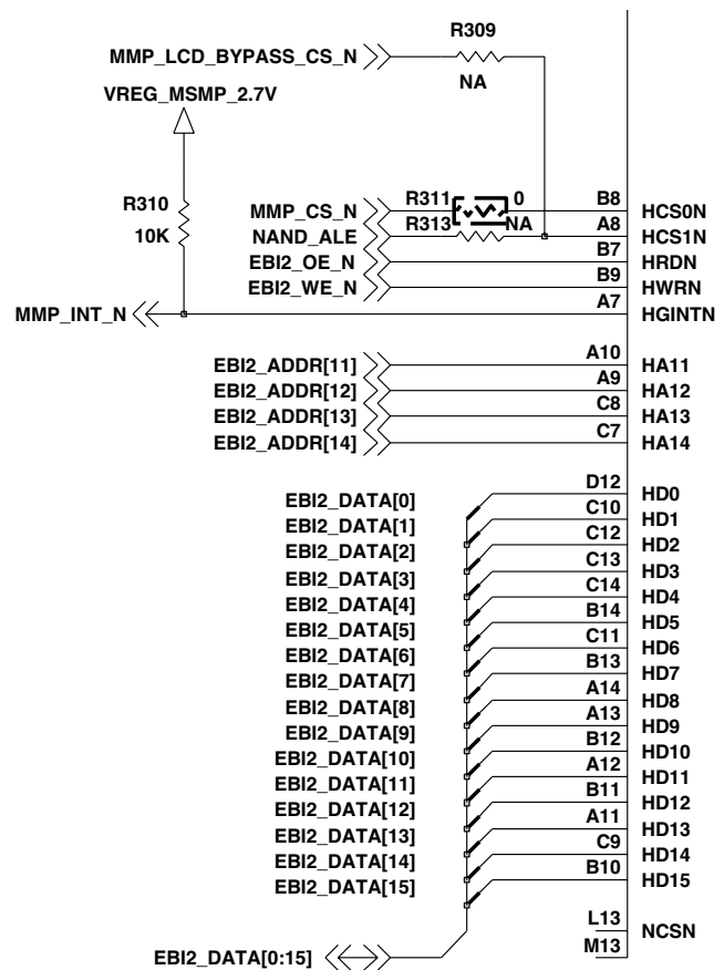
[ Schematics ]
