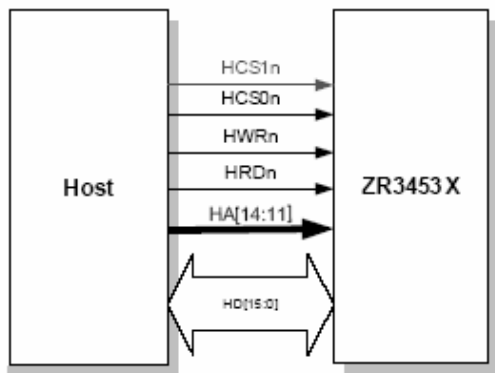
[ Block Diagram ]
