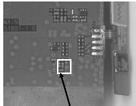
C567, C568
