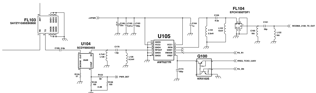
[Figure 1.5] UMTS PAM, Duplexer, Coupler
