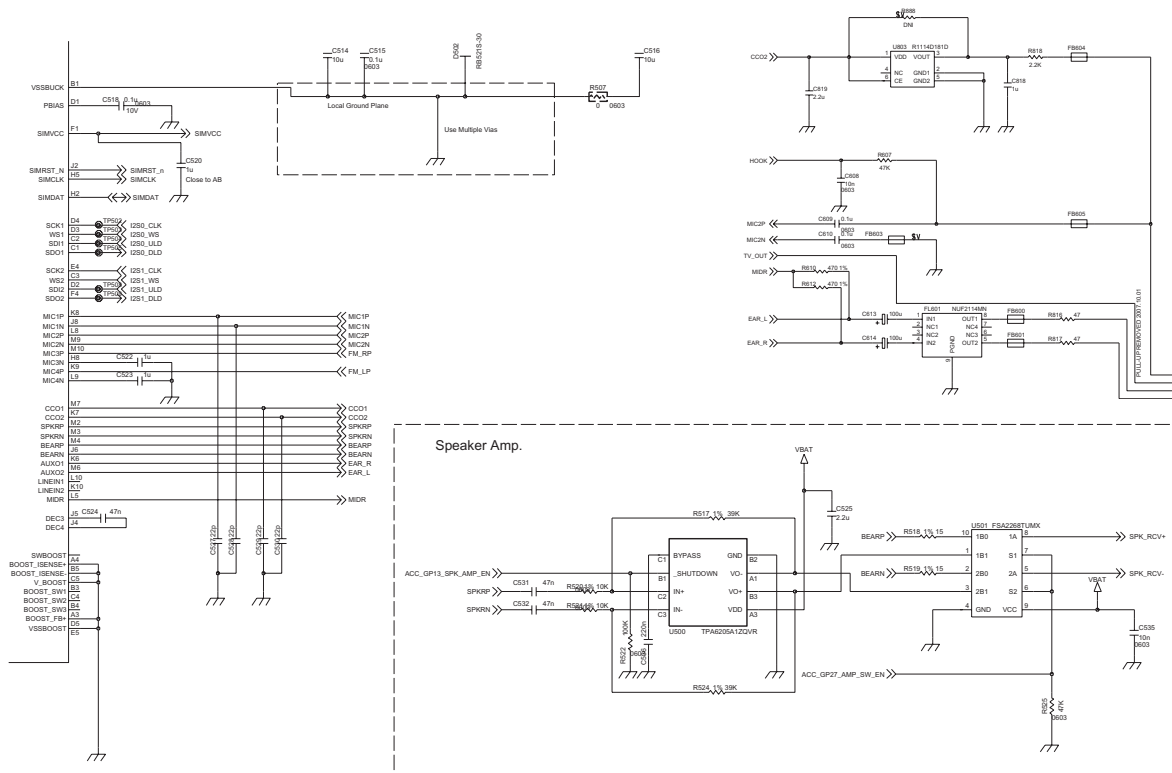
Figure 3-3-3 . Audio Section scheme
