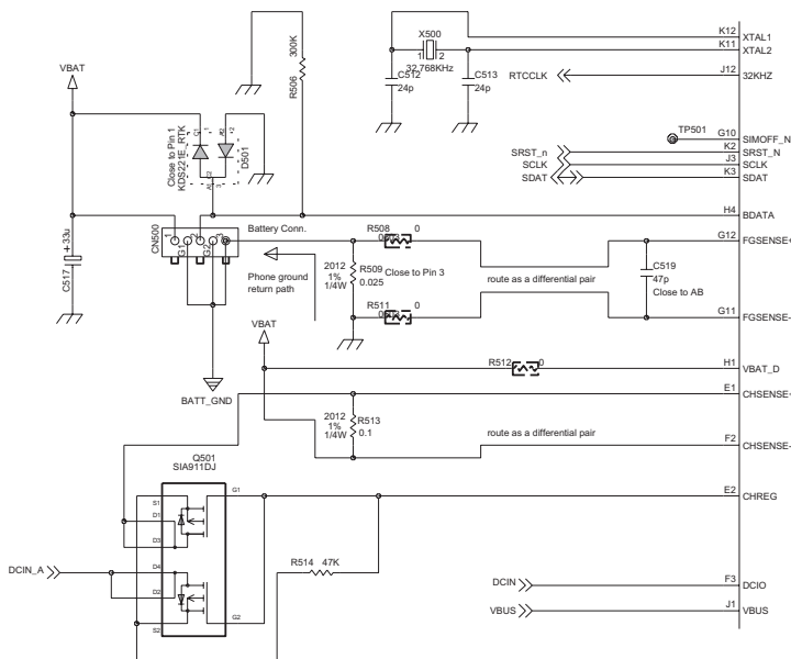
Fig. 3-5-1. Battery charging circuit
