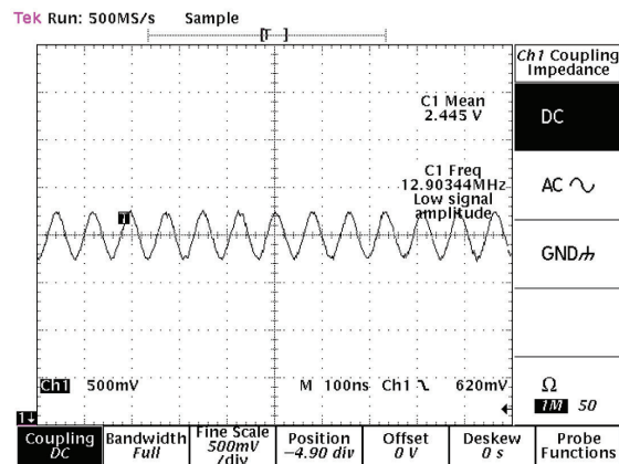
Figure 4-13. 26MHz at R114
