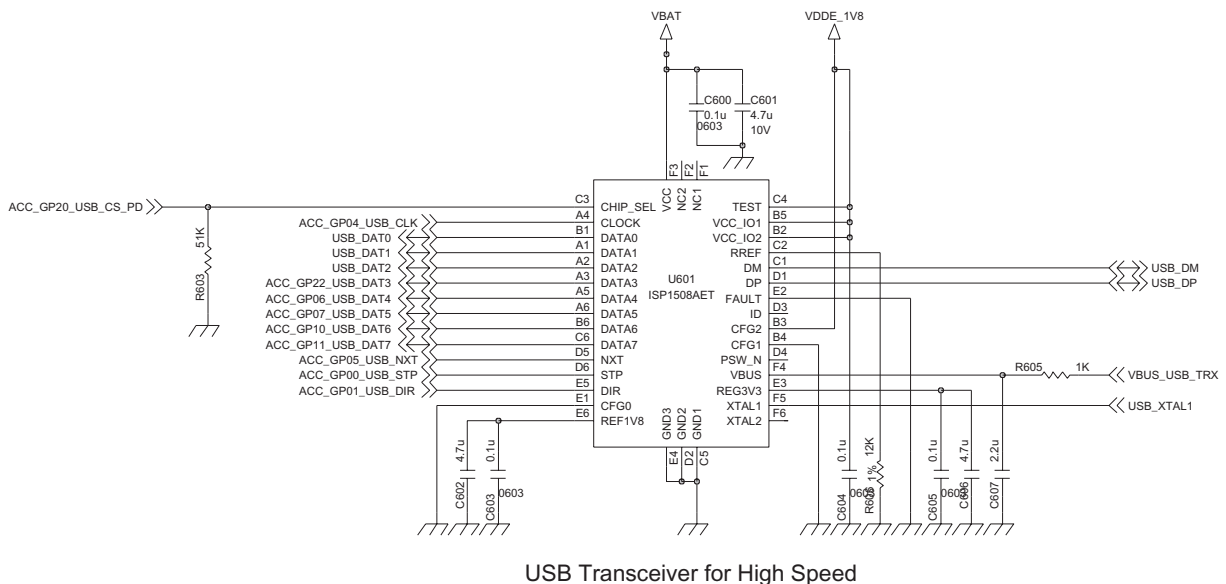
Figure 3-1-9. Schematic of USB Transceiver
