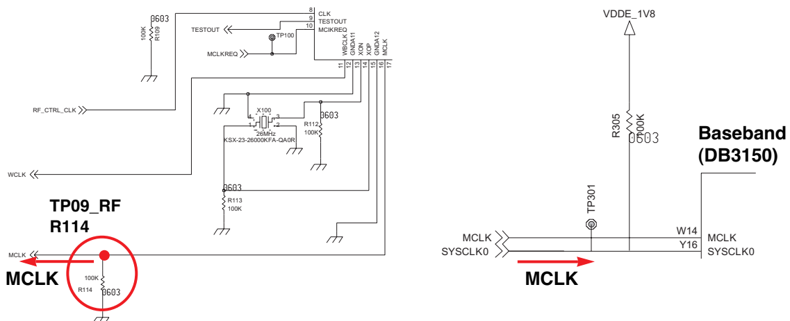
Figure 4-12-2. Schematic (26MHz at BB Part)
