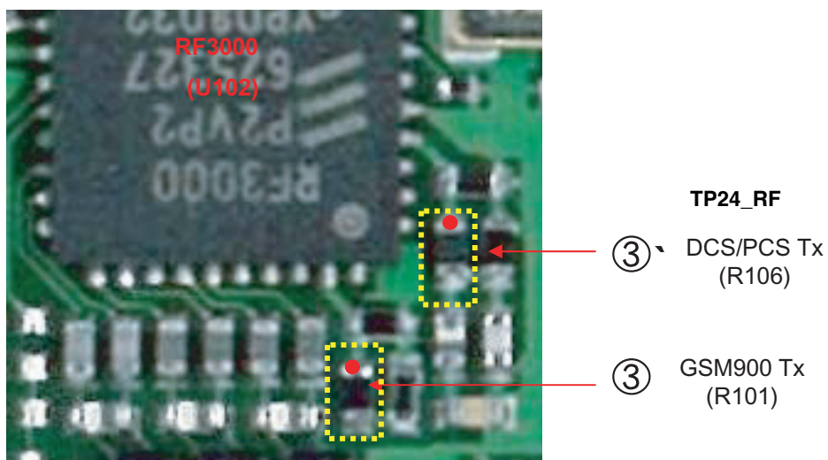
Figure 4-19. GSM900/DCS/PCS Transceiver (RF3000)
