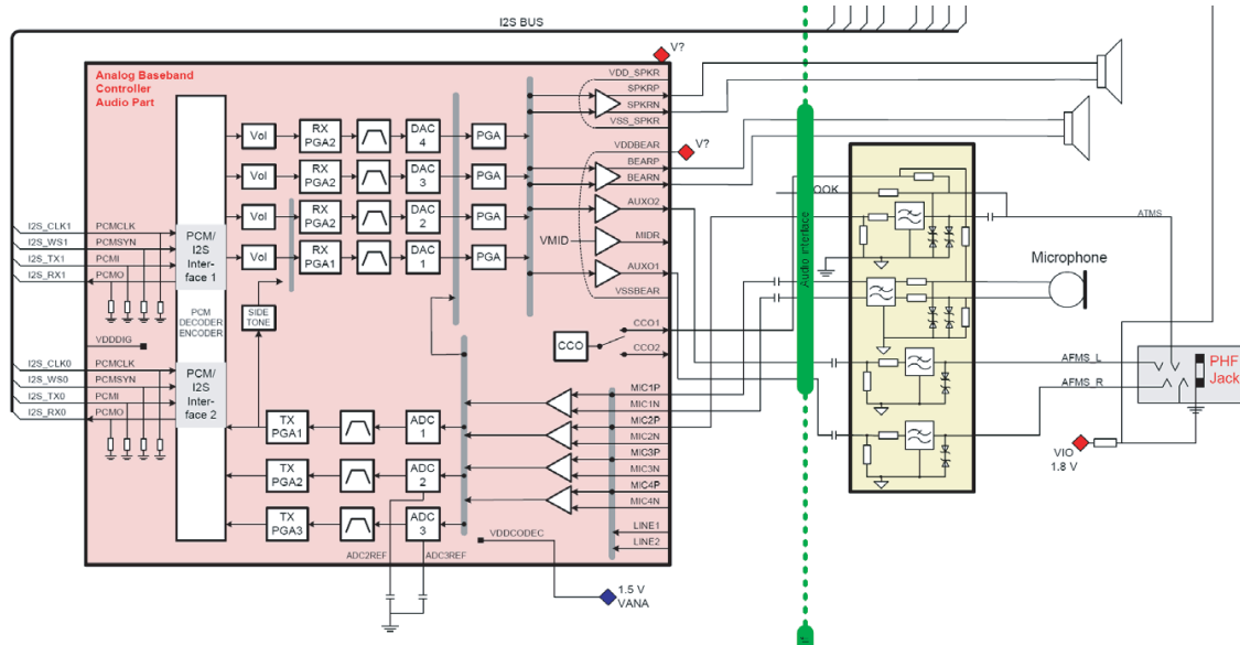
Figure 3-3-2. Audio Interface Detailed Diagram(Veronica)
