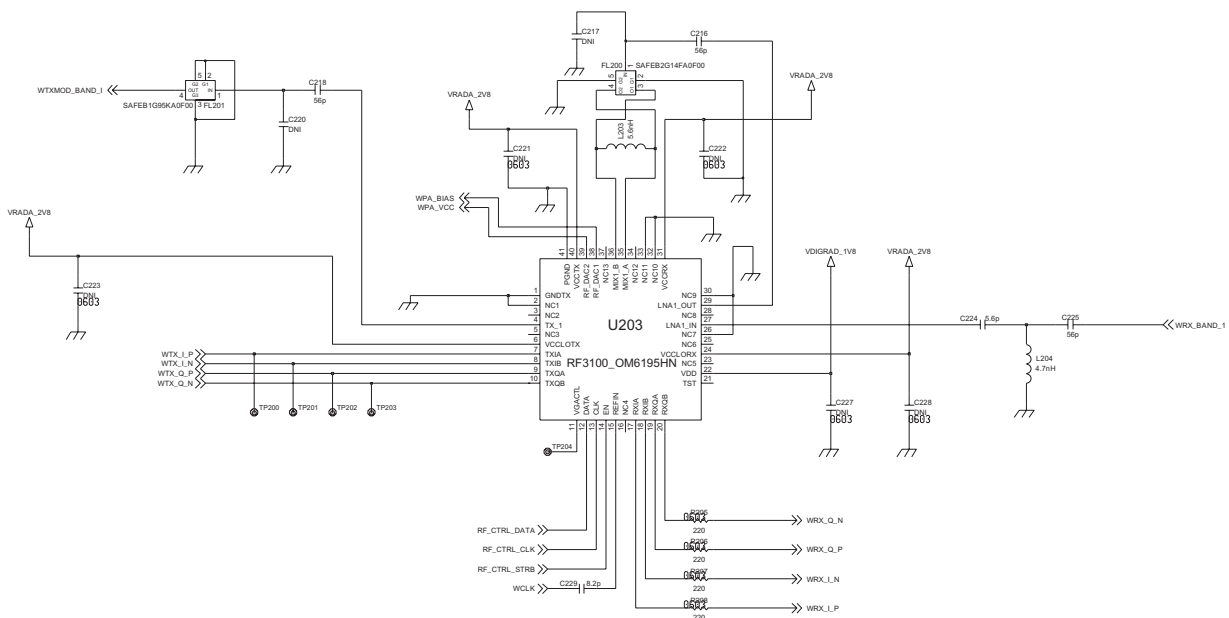
Figure 3-7-4. WCDMA Transceiver schematic
