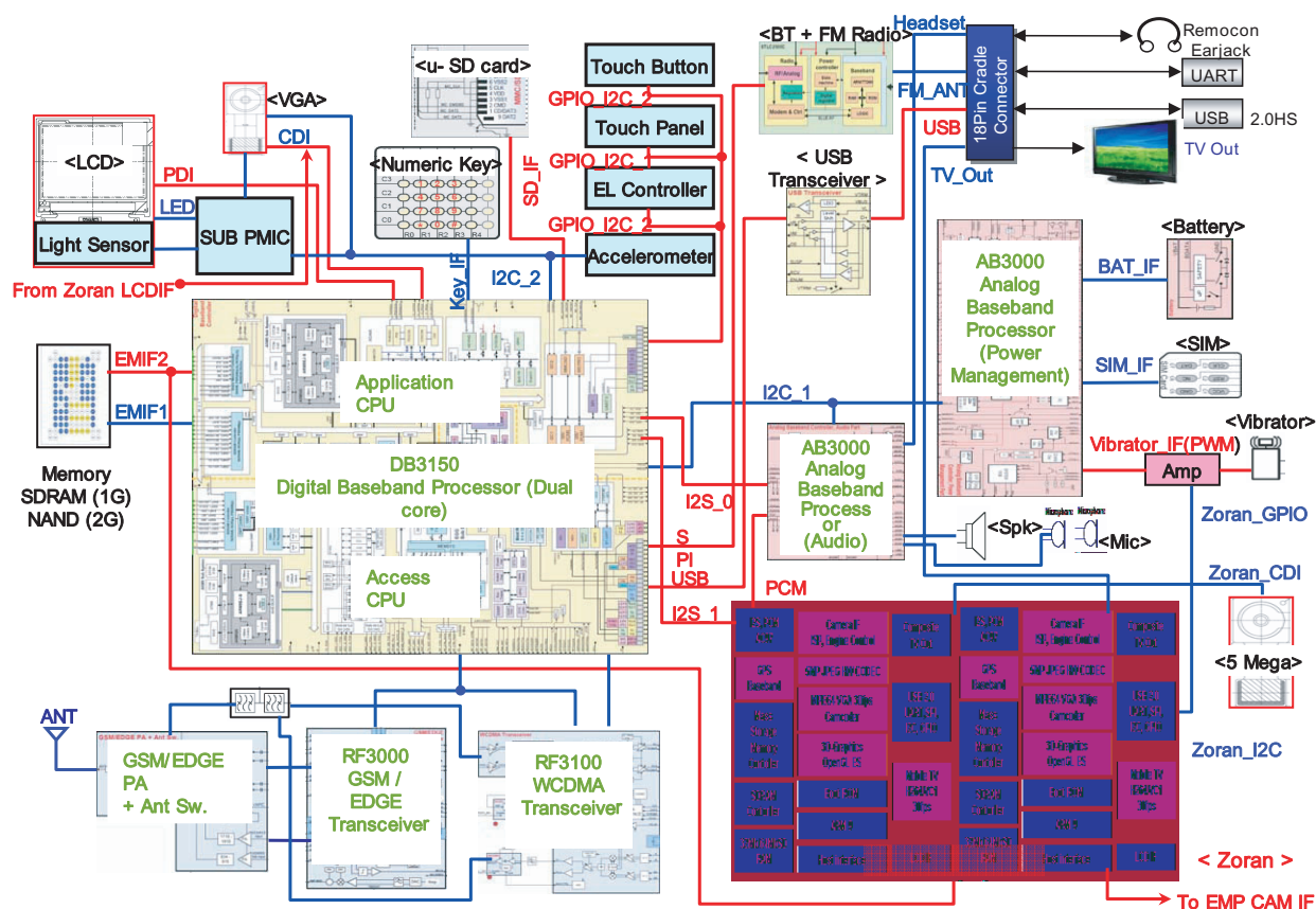
Figure 3-1-1 KF750 Block Diagram
